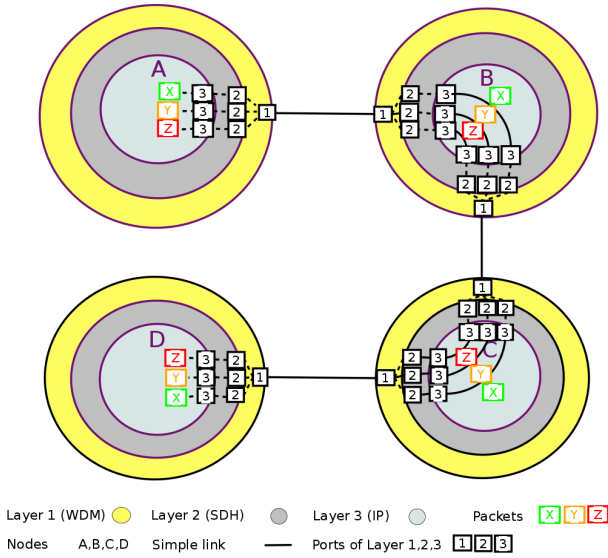
FIGURE 3: IP over SDH over WDM
