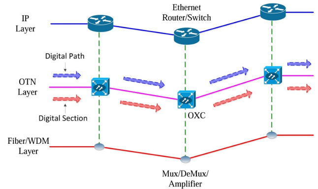
FIGURE 2: OTN based layered network architecture
